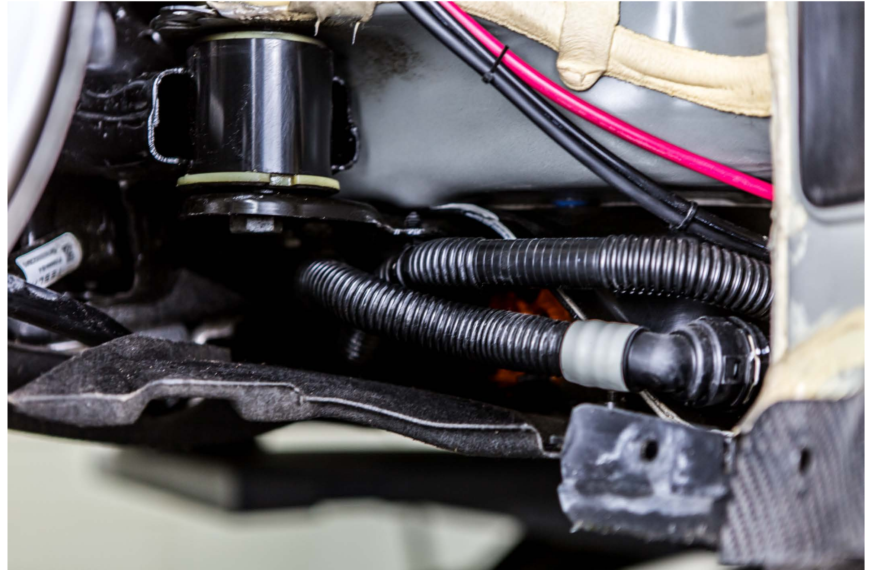
Rear Right Illustration Route Airline, Height sensor cable and power lines through the rear right wheel area
