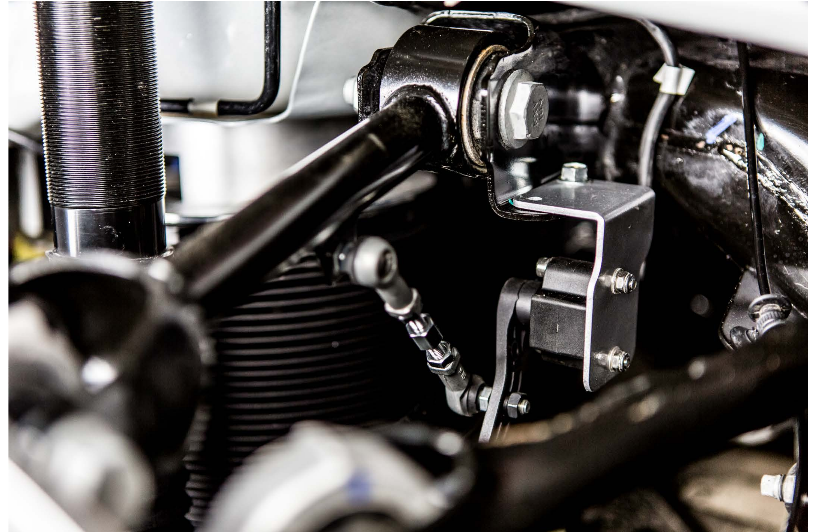
Rear Right height sensor Install the bracket on the rear right control arm. Mount it on the inside bolt
